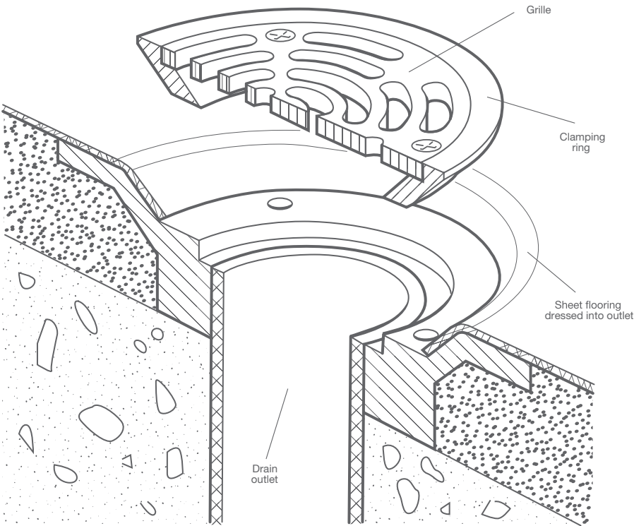
Transition with clamping drain
