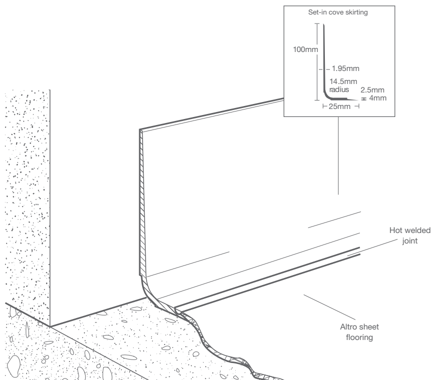
Set-in cove skirting
