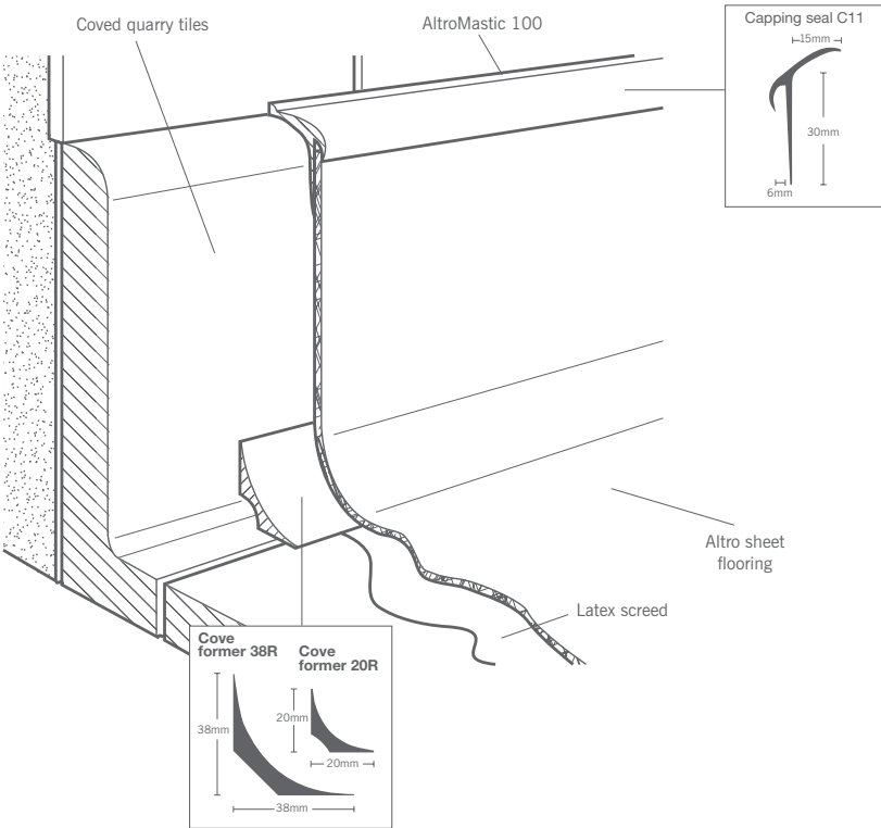
Self-coved with cove former and capping seal C11 over floor tiles
