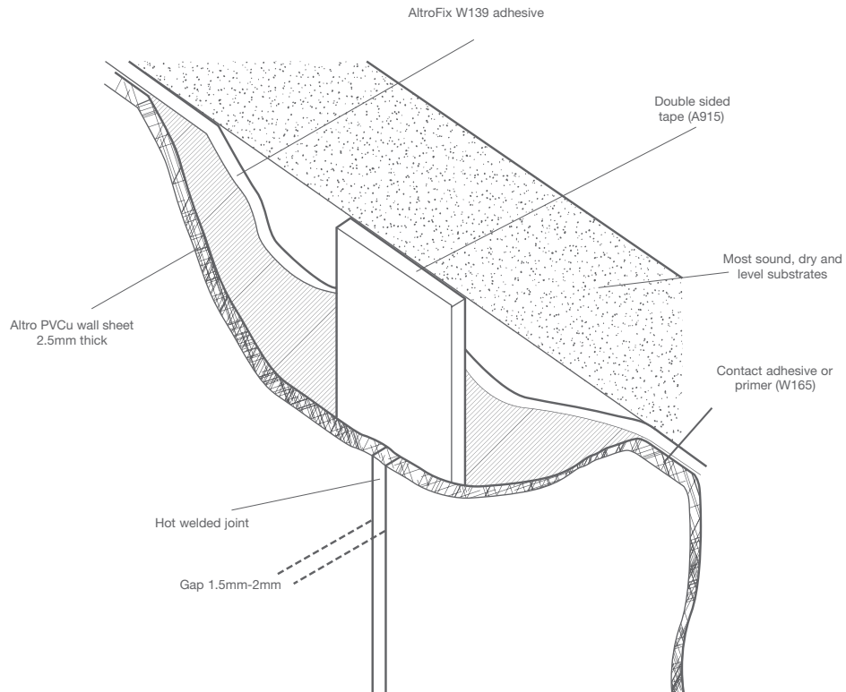
Altro wall sheet to Altro Whiterock FlexiJoint detail
