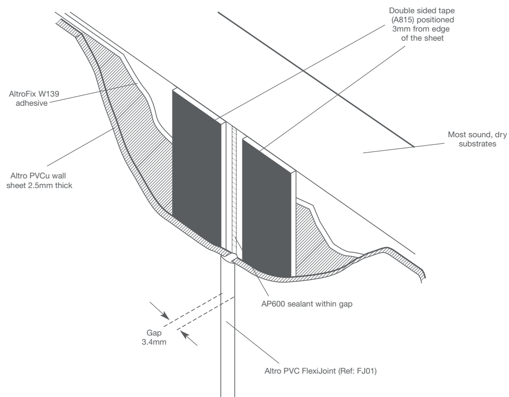
Altro wall sheet to Altro Whiterock FlexiJoint detail
